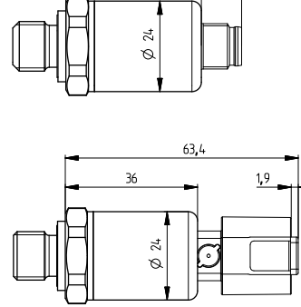
M12x1
