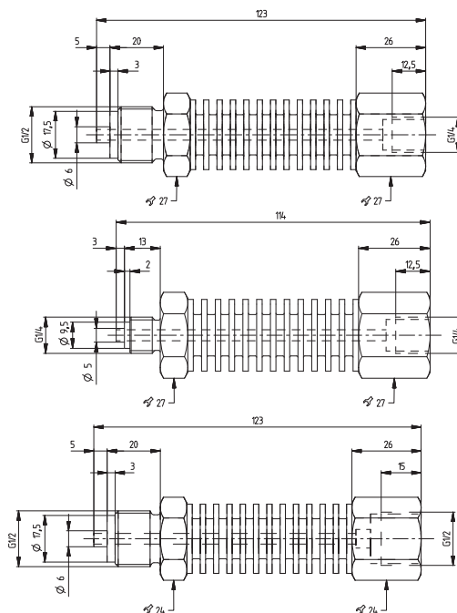
Heat sink
