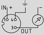
Connector M12x1
