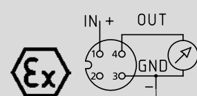
Connector M12x1
