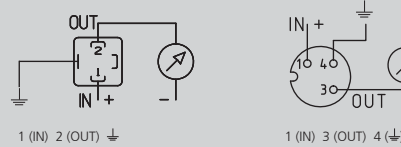
1 (IN) 2 (OUT) 1 (IN) 3 (OUT) 4 (GND)
