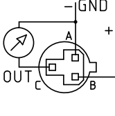
B (IN) C (OUT) A (GND)
