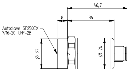
7/16 - 20 UNF-2B / M12x1
