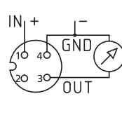
1 (IN) 3 (OUT) 4 (GND)
